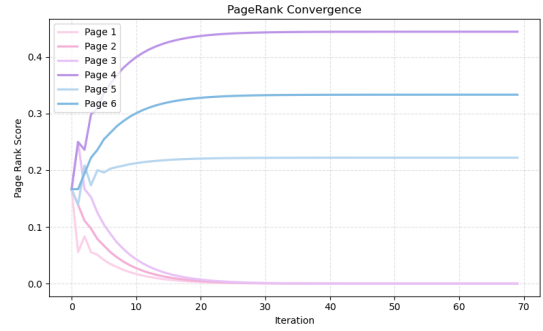
Figure 1. PageRank convergence for graph 1.
