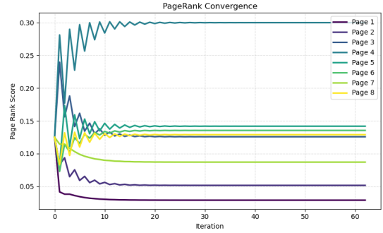
Figure 2. PageRank Convergence for graph 2.
